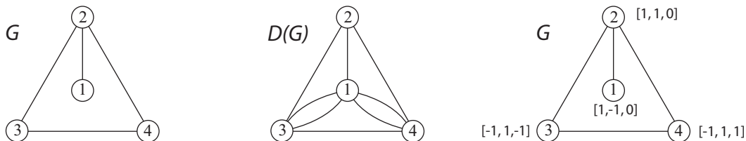
Figure 2: A graph G , its distance multigraph D(G) , and an addressing of G obtained from the edge-disjoint biclique decomposition of D(G) in Figure 1.
