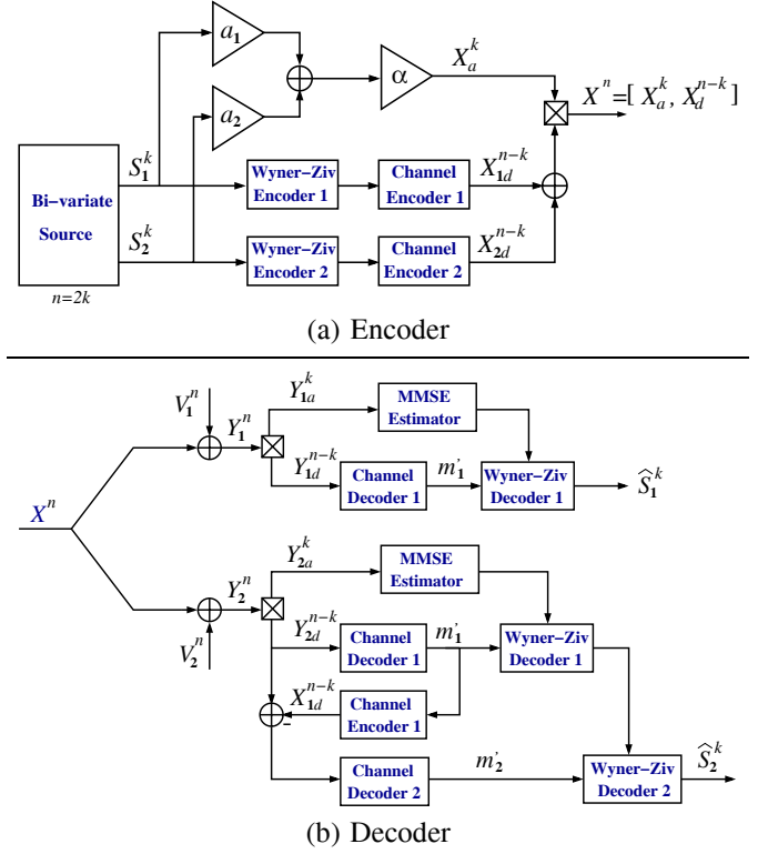
Fig. 3. Broadcasting a bivariate source S^k = (S_1^k, S_2^k) with bandwidth expansion: the HWZ scheme.
