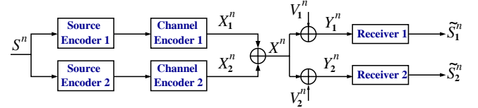
Fig. 1. Broadcasting a single memoryless Gaussian source using separate source-channel codes. Source encoder 1 is an optimal encoder with rate R_1 , source encoder 2 is an optimal encoder for the residual error of encoder 1 with rate R_2 - R_1 . The two codes are superpositioned and transmitted across a power-limited Gaussian two-user broadcast channel.
