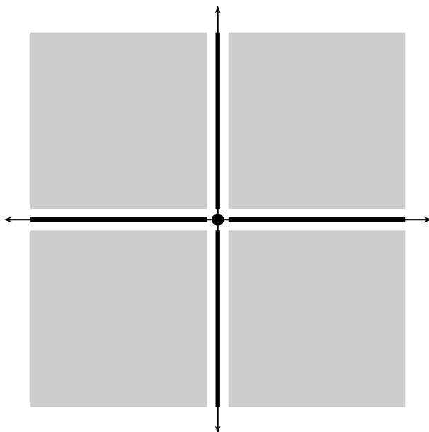
Figure 4. Integral manifolds
