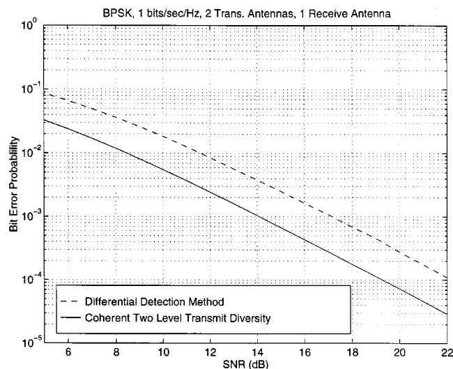
Fig. 3. Performance of the differential detection and coherent detection: two-level transmit diversity scheme for BPSK constellation.
