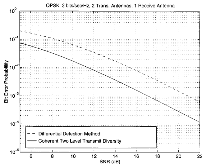
Fig. 4. Performance of the differential detection and coherent detection: two-level transmit diversity scheme for QPSK constellation.
